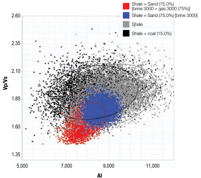
Figure 6. Stochastic forward modelling from the depths of X to X + 600 m combined. Consider the point at the position AI=8,500 and Vp/Vs=1.65. On this plot the probability of it being hydrocarbon, brine or shale is roughly equal. In Figure 5 the same point has an overwhelming probability of being hydrocarbon.
