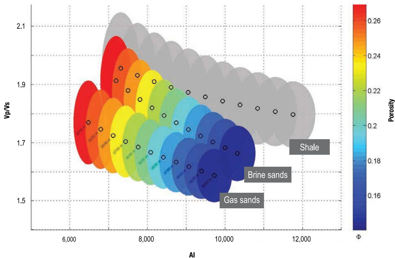
Figure 7. A plot of AI vs Vp/Vs for varying depths and porosities. Ellipses are illustrative of ~1 standard deviation of scatter. Ellipse rotation is not accounted for in this figure. Fluid discrimination is good at all depth levels, however does decrease with increasing depth. Fluid and lithology discrimination is maximised using both P and S attributes. Lithology discrimination increases with depth.
