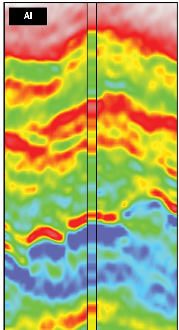
Figure 11. Acoustic impedance tie at one of the wells.
