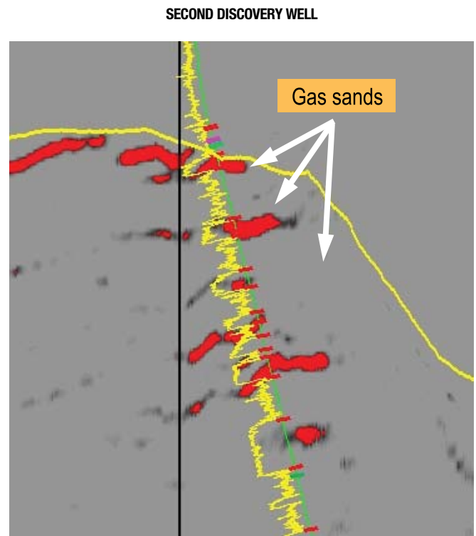
Figure 16. A cross section through the gas probability volume at the second discovery well.
