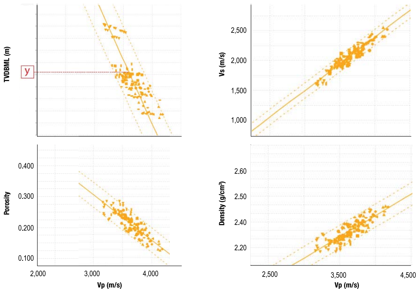
Figure 4. Sand trends for the area. As for the shales, each point represents an interpreted, upscaled end member interval.
