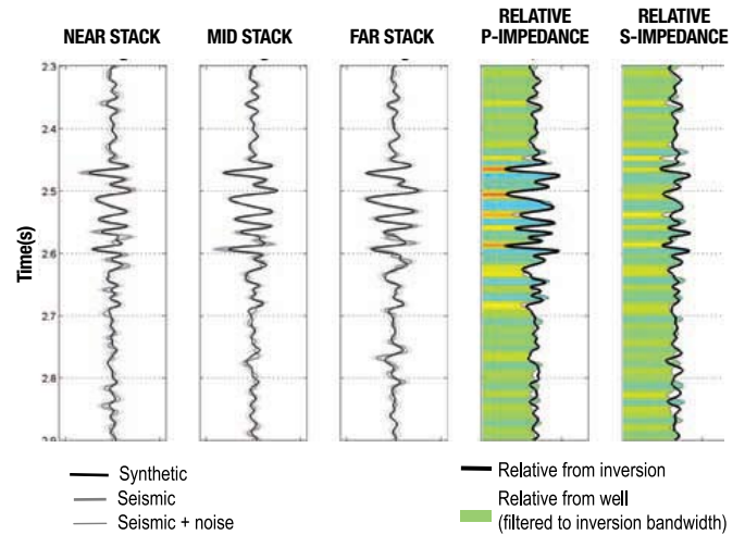
Figure 10. Relative impedance ties at one of the discovery wells.
