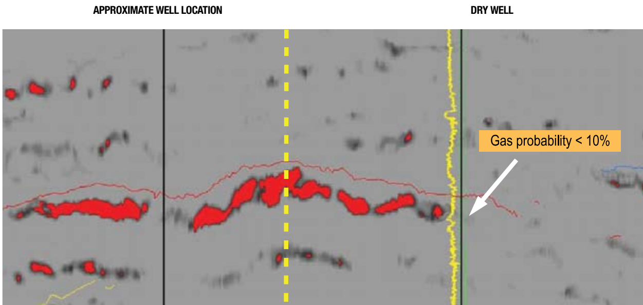
Figure 17. Third well, third discovery. Arblines showing discovery well position along with previous dry hole.
